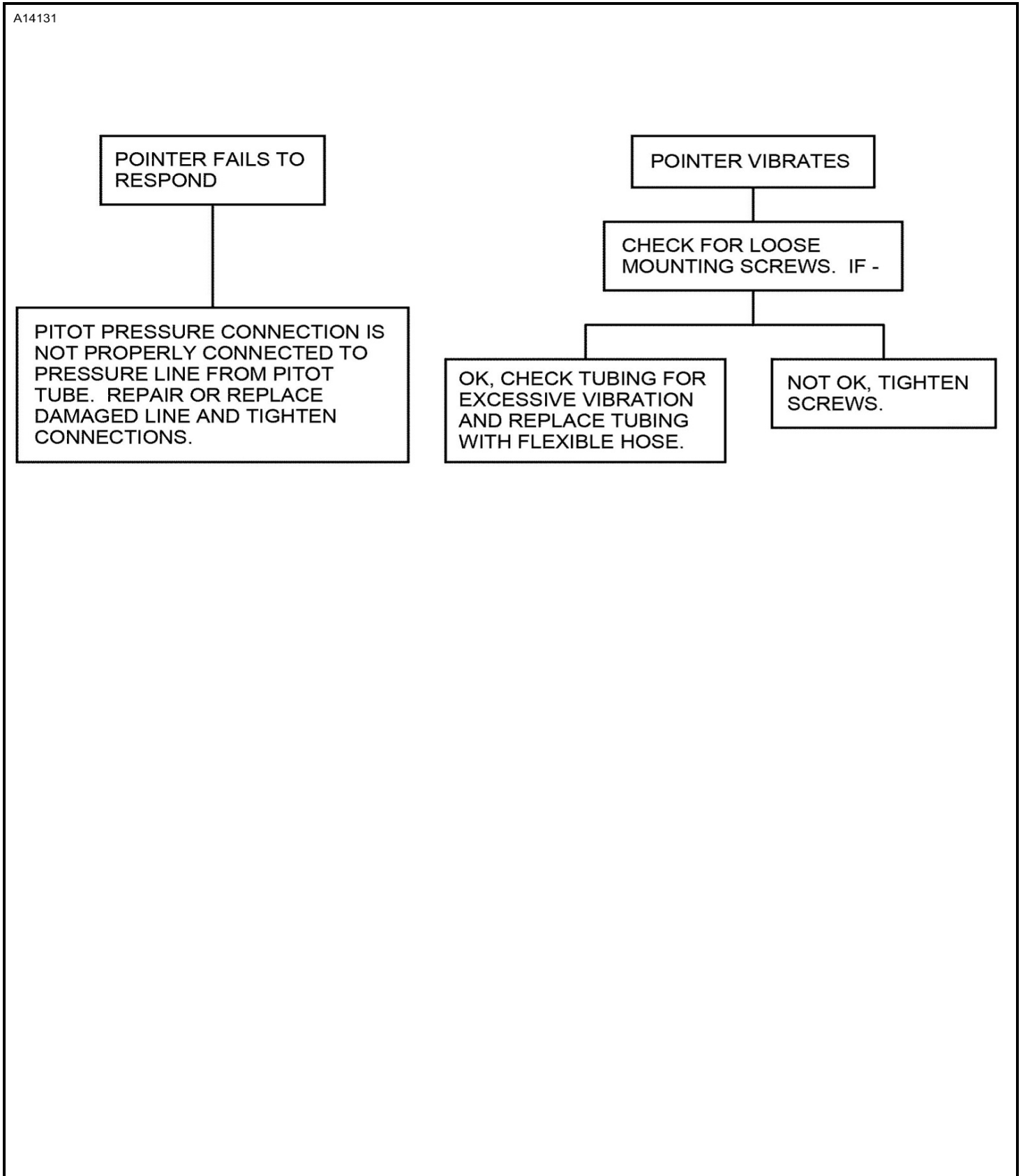
Figure 101 : Sheet 2 : Airspeed Indicator Troubleshooting Chart
